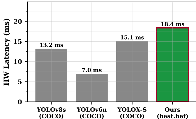
(b) Single-Inference NPU Latency Hailo-8L NPU
